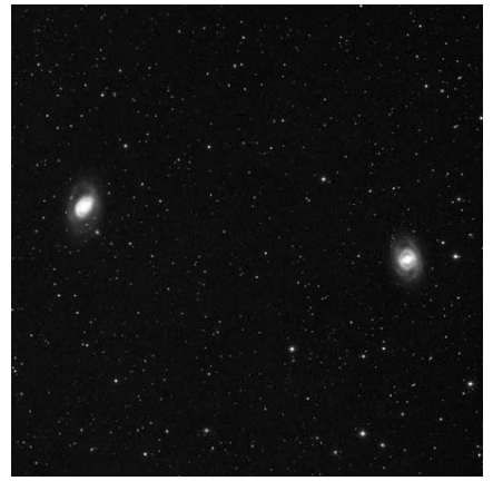
M95 & m96
