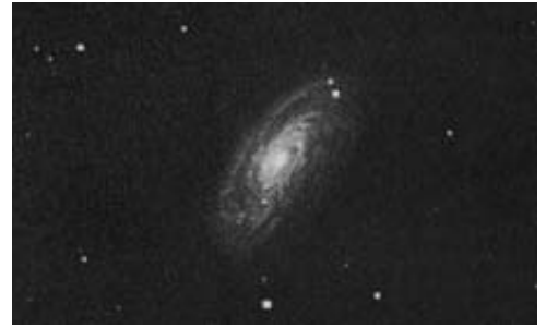
M88
